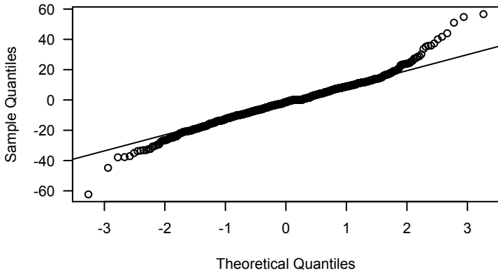
difference in % change dBP Q-Qplot
