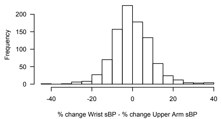
difference in % change sBP histogram
