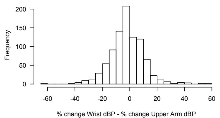
difference in % change dBP histogram
