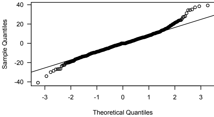
difference in % change sBP Q-Qplot
