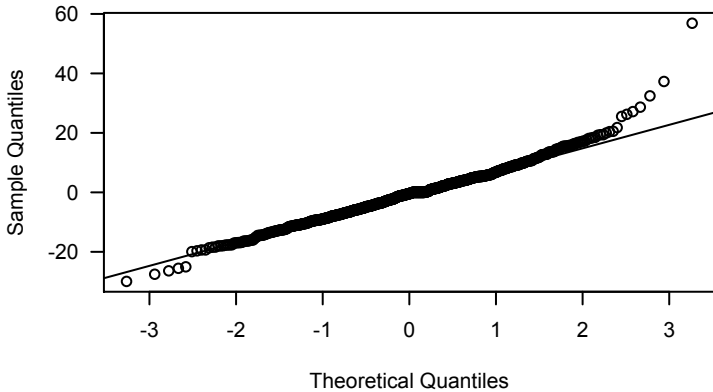
difference in % change mBP Q-Qplot
