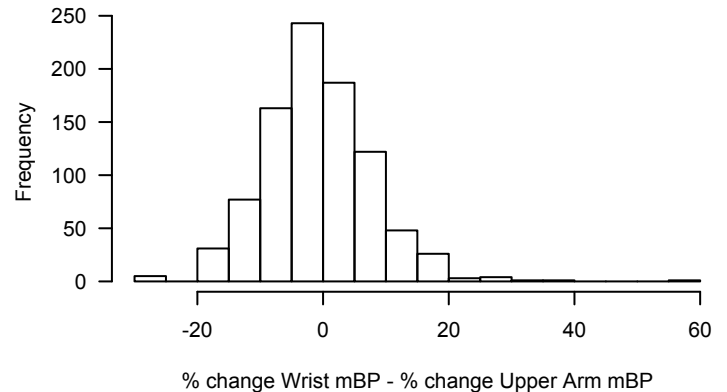
difference in % change mBP histogram
