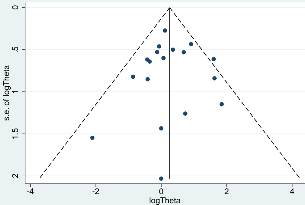
Funnel plot with pseudo 95% confidence limits for Figure 6
