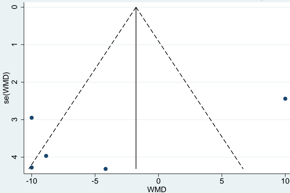
Funnel plot with pseudo 95% confidence limits for Figure 4
