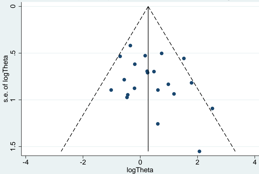
Funnel plot with pseudo 95% confidence limits for Figure 5
